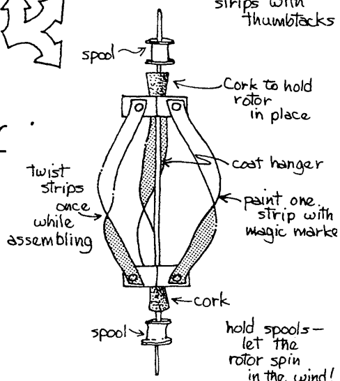
Helix Rotor
