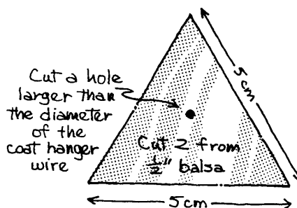
Helix Rotor
